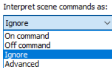
Figure 7.: Scene Interpretation
